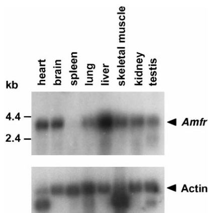
Fig. 3. (A) Northern blot analysis of the Amfr gene in various mouse tissues. Mouse MTN Blot (Clontech) was hybridized with an Amfr cDNA probe. A mRNA transcript of 3.5 kb is indicated by an arrowhead. The membrane was re-hybridized with a human \beta -actin probe.
