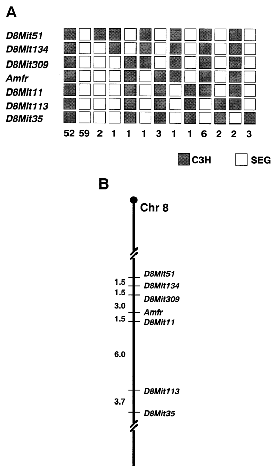
Fig. 4. (A) Haplotype data of 134 progenies of (C3H/HeJ \times SEG) F1 \times C3H/HeJ for the loci flanking the Amfr locus. The microsatellite and Amfr loci are listed at the left. Each column represents a chromosomal haplotype identified in the progenies. Filled box, C3H/HeJ allele; open box, SEG allele. The number of progenies for each haplotype is listed at the bottom of each column. (B) A genetic map around the Amfr locus constructed from the haplotype data. Recombination frequencies expressed as genetic distances in cMorgans are shown on the left.
